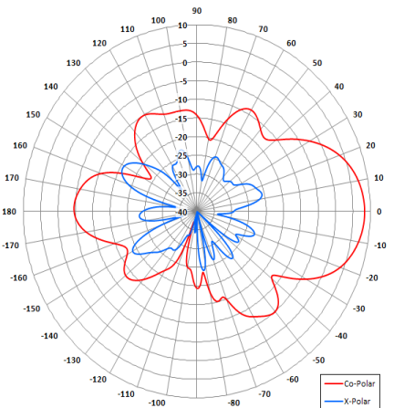
Elevation Pattern - Sector
