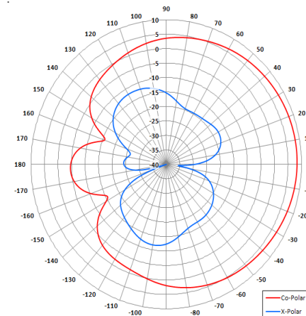
Azimuth Pattern - Sector
